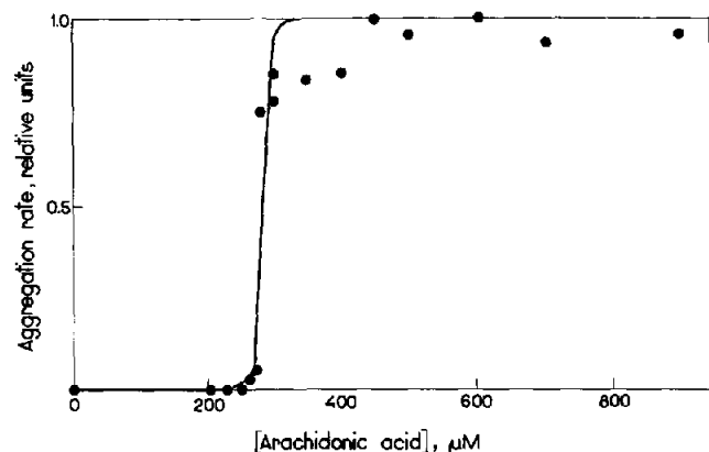
Fig. 2. Relationship of the rate of arachidonate-induced human platelet aggregation to the concentration of the inducer. The theoretical curve is plotted using Eq. (1) ( K_A = 275 \mu M, h_A = 30 ).
