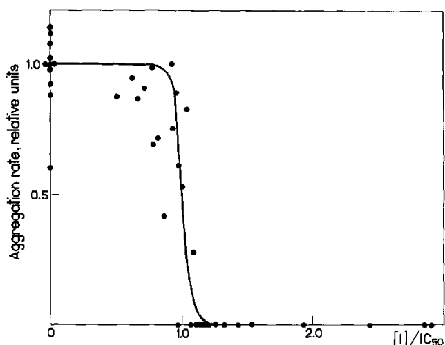
Fig. 1. Relationship of the rate of arachidonate-induced human platelet aggregation to the concentration of 3-(3-pyridyl)-5-phenylisoxazole. Arachidonic acid, 500 \mu M. The theoretical curve is plotted using Eq. (2) ( h_1 = 30 ).
